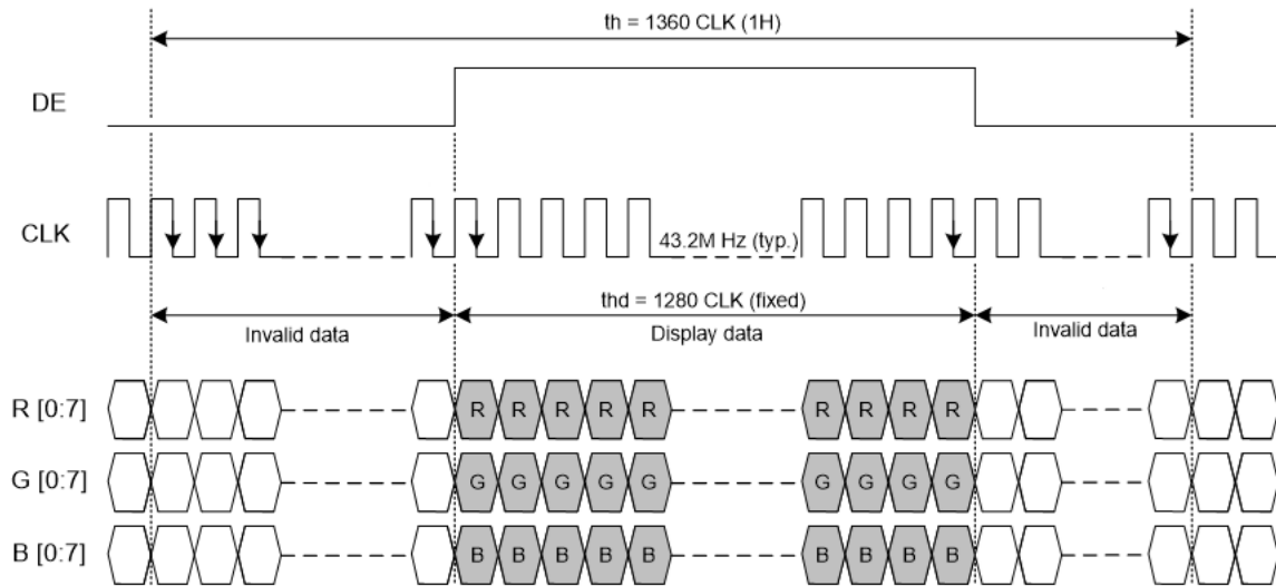
Fig. 9.1 Horizontal Timing
