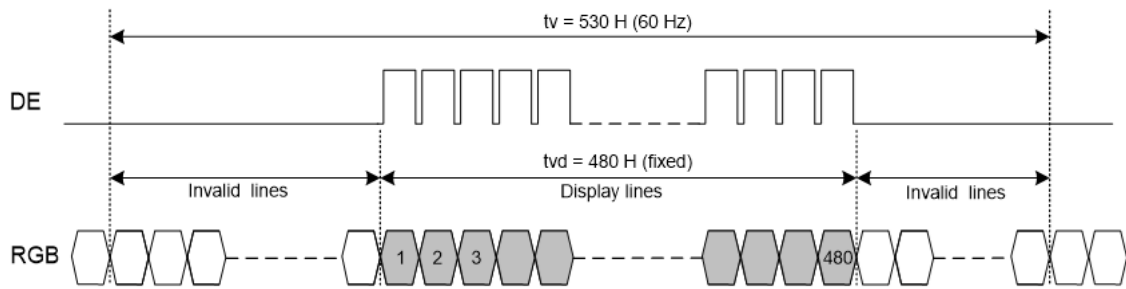
Fig. 9.2 Vertical Timing
