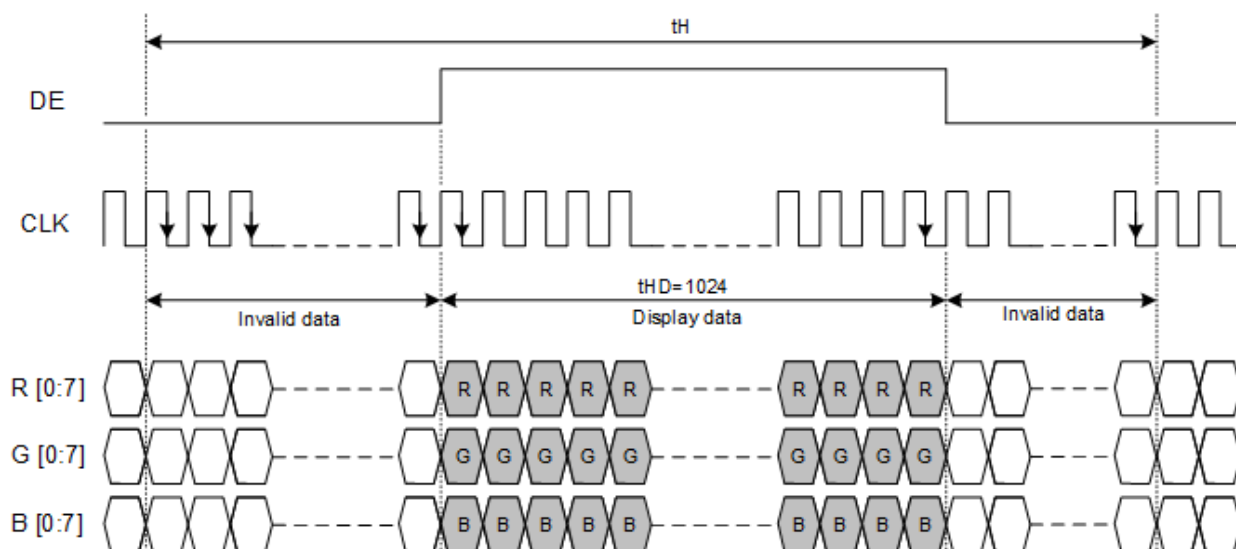
Horizontal timing
