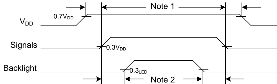
Fig 9.4 Power Sequence
